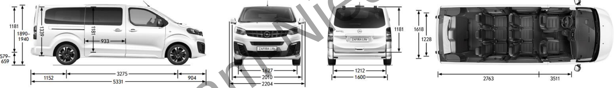
Zafira Electric XL Alle Maße in mm
