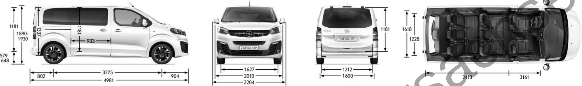
Zafira Electric Alle Maße in mm
