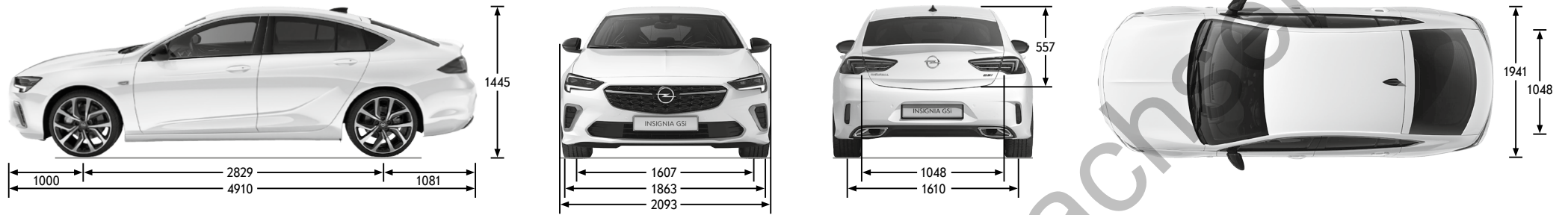
Grand Sport Alle Maße in mm
