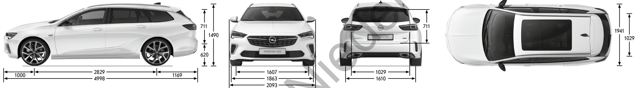
Sports Tourer Alle Maße in mm
